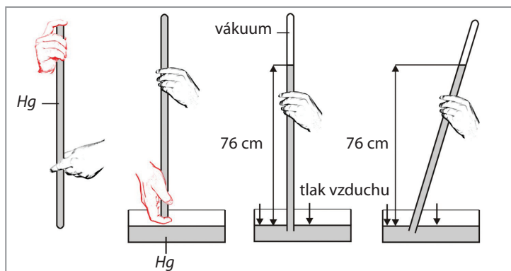
Obr. 95 Torricelliho pokus
